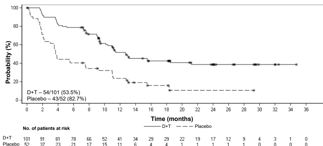
Figure 5 Kaplan-Meier PFS curves for Study J12301 (primary analysis)
