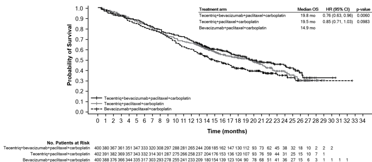
Figure 4: Kaplan-Meier curve for overall survival in the ITT population (IMpower150)
